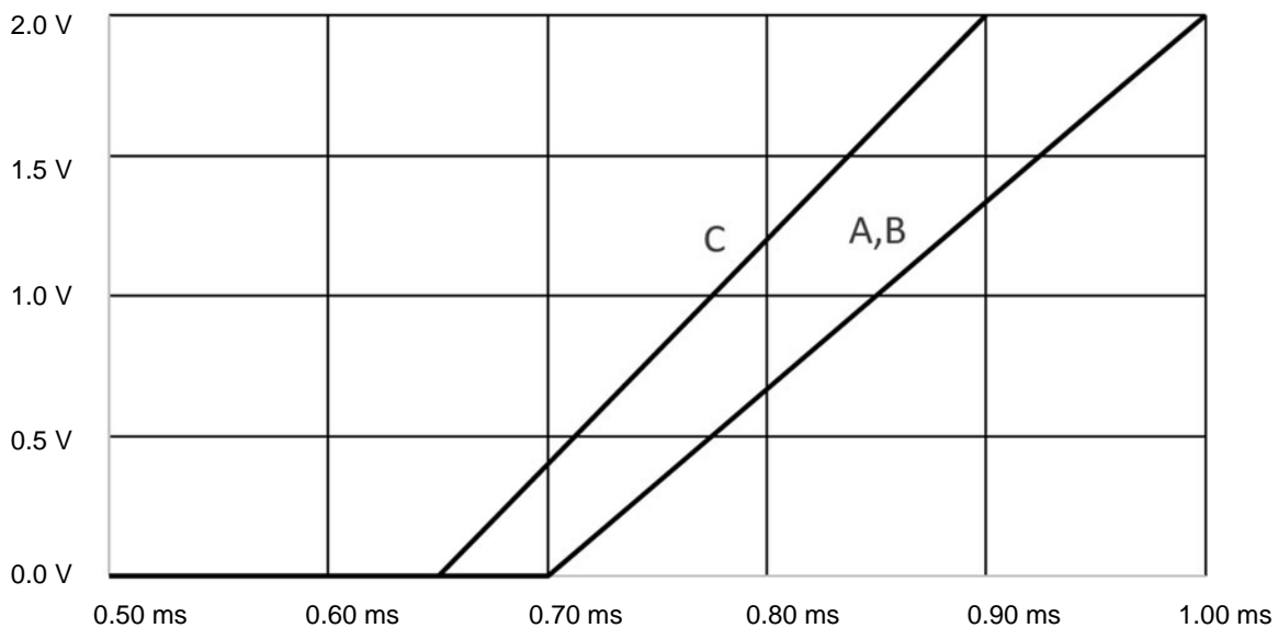
Voltage correction of long OSSD test pulses
